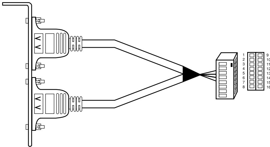
Dual Series A Receptacle to 2.54mm 16 Position Connector
