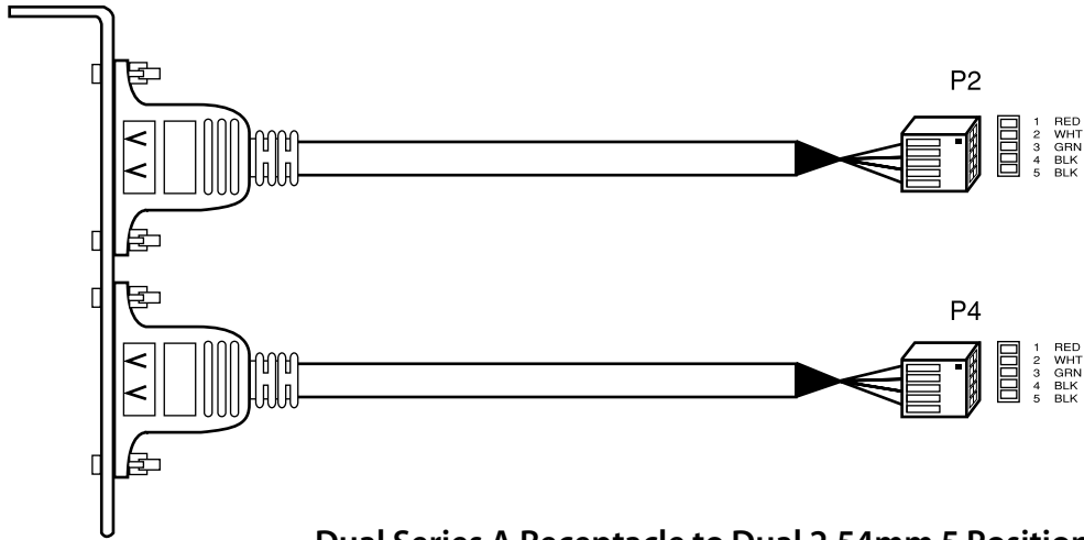
Dual Series A Receptacle to Dual 2.54mm 5 Position Connectors
